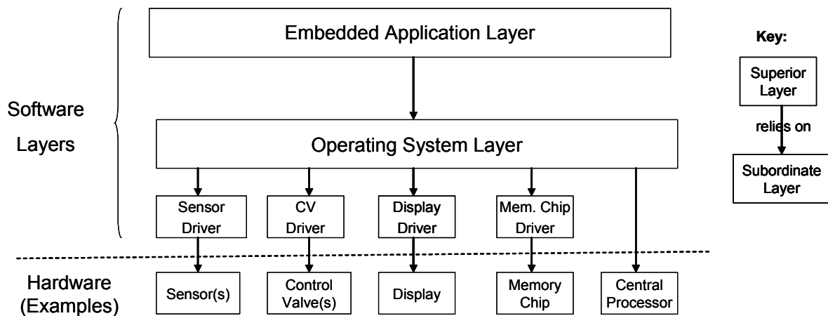
Figure 2.2.3.2 - Typical layered architecture for a real-time embedded-software computer system
