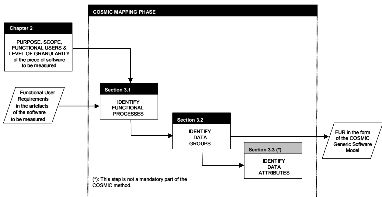
Figure 3.0 – General method of the COSMIC mapping process
