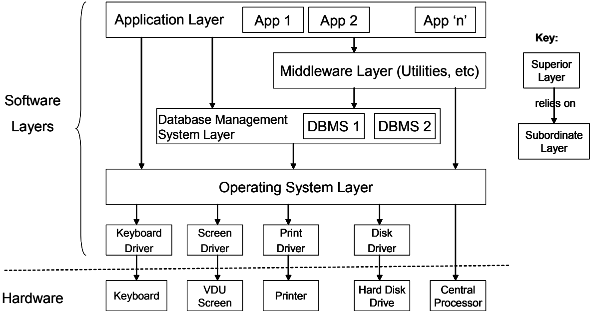
Figure 2.2.3.1 - Typical layered software architecture for a Business/MIS computer system
