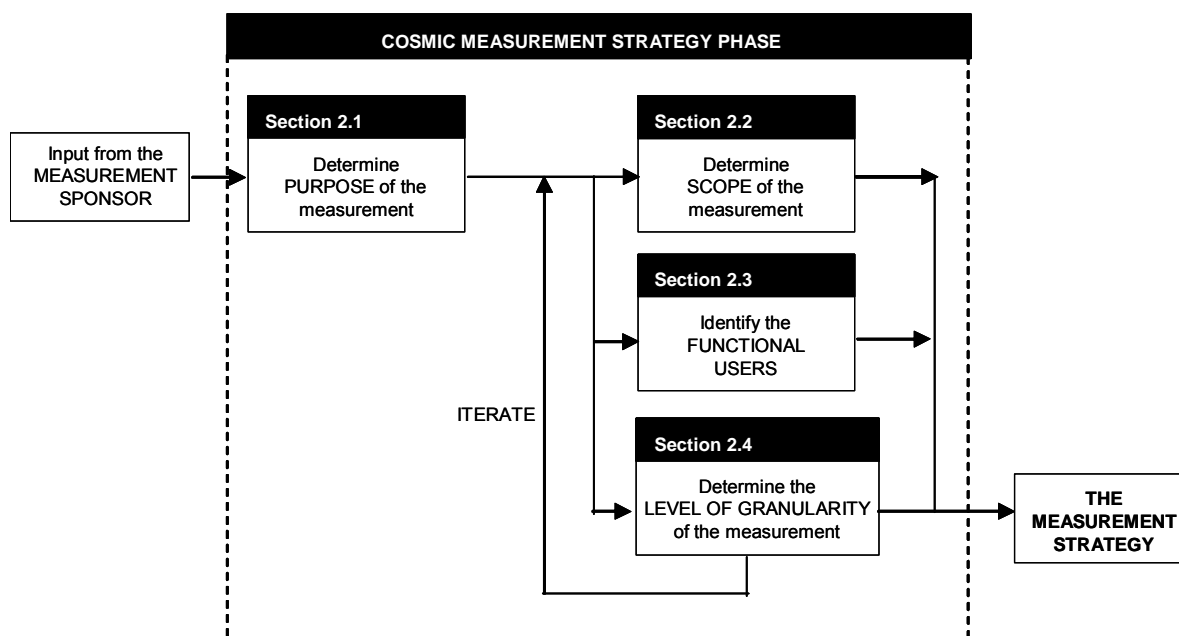
Figure 2.0 - The process of determining a Measurement Strategy
