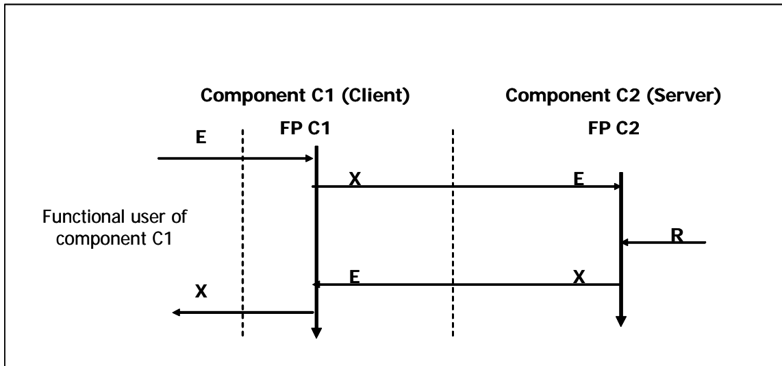
Figure 4.1.8.2 Data exchanges between peer components in the same layer
