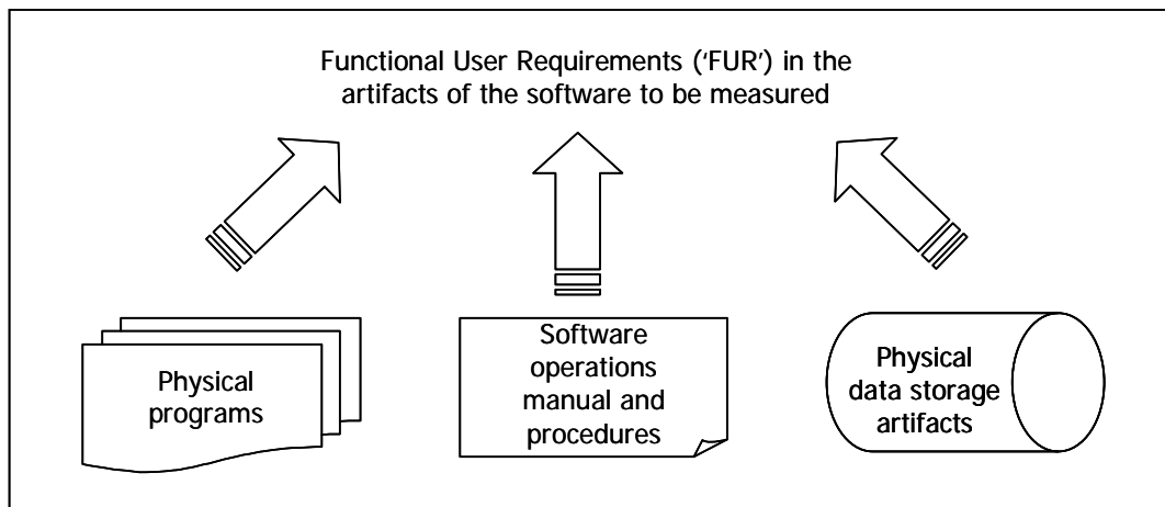
Figure 1.2.2. – COSMIC model of post-implementation functional user requirements
