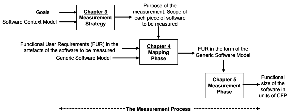
Figure 1.5 – Structure of the COSMIC method
