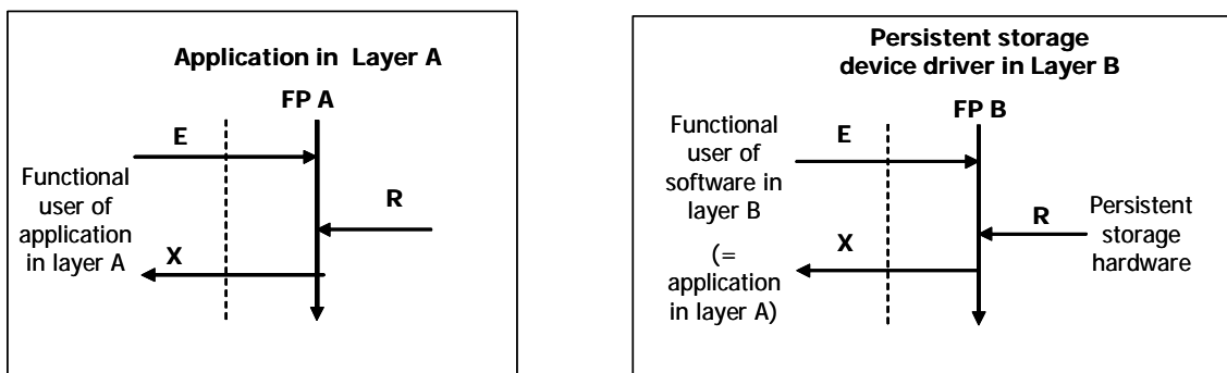
Figures 4.1.8.1 (a) and (b) Solution for a Read issued by software 'A' in the application layer to software 'B' in the device driver layer
