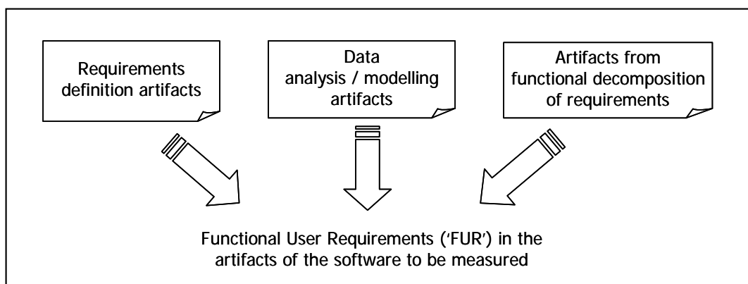
Figure 1.2.1 – COSMIC model of pre-implementation functional user requirements
