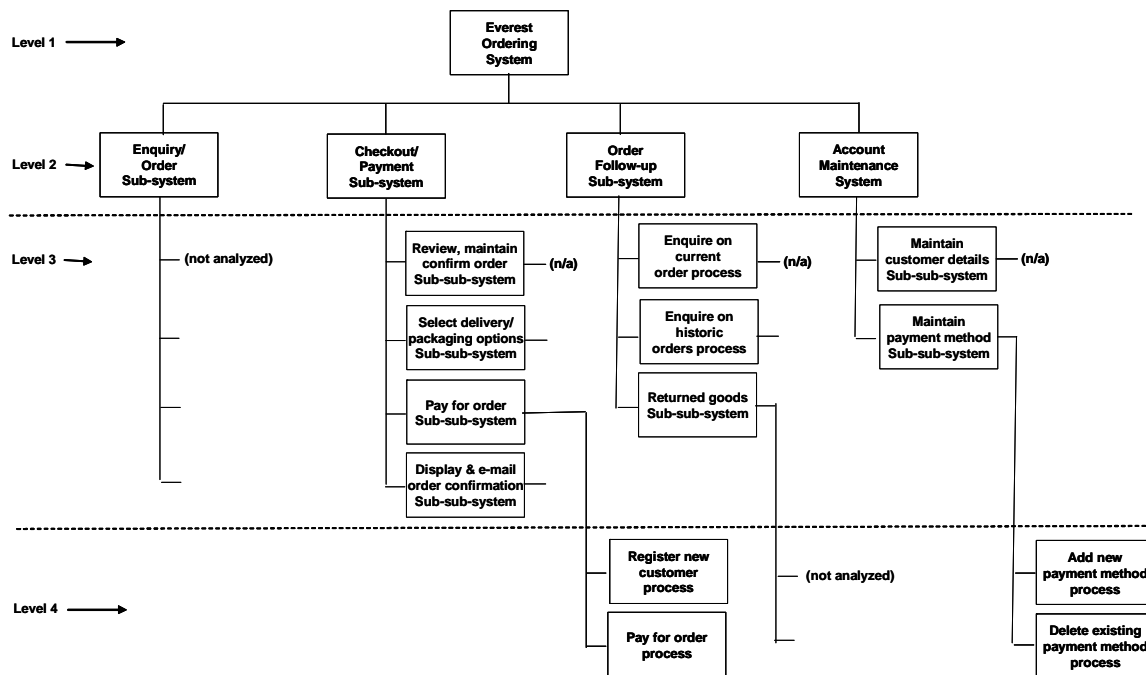
Figure 2.4 - Partial analysis of the Everest Ordering System showing four levels of analysis
